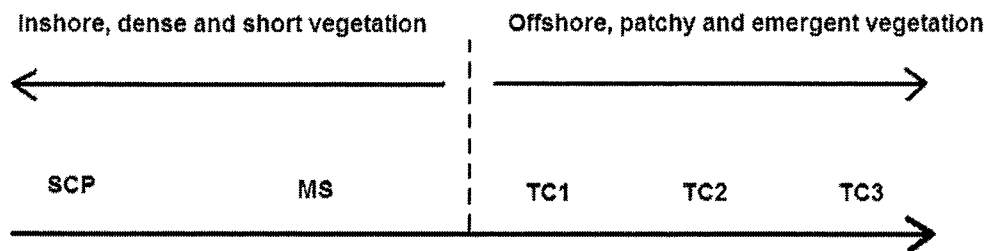
Fig. 1. The microhabitat gradient at Isterhäset: SCP = "short Carex and Poaceae ", MS = "muddy shore", TC = "tall Carex " in three categories ordered by increasing height and patchiness and decreasing overall density (TC 1 => TC2 => TC3). Out of the total hydrolittoral in area L, SCP made up 34.5%, MS 2.0%, TC1 38.0%, TC2 6.4%, and TC3 19.0%.
